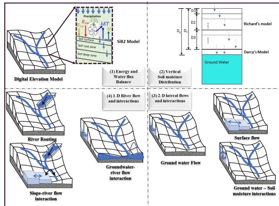
Figure 5. Schematic diagram of the water and energy balanced-based rainfall–runoff–inundation (WEB-RRI) model and its four major modules. Reprinted with permission from Ref. [48].
